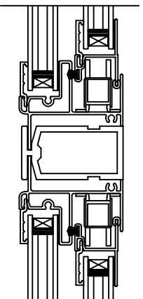
CHS Twin/Triple Intermediate Jamb Detail
