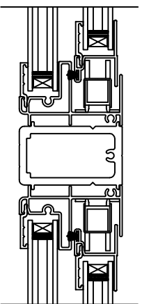
CHS Twin/Triple Intermediate Jamb Detail
