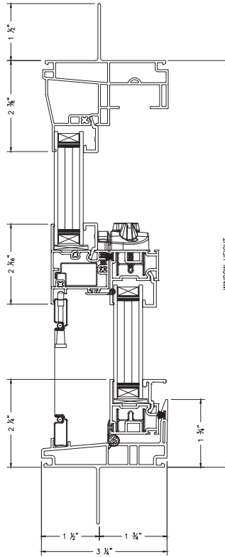
4300 SINGLE HUNG VERTICAL CROSS SECTION
