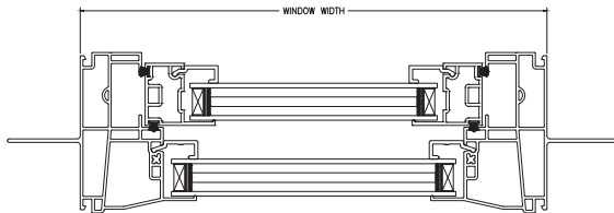
4300 SINGLE HUNG HORIZONTAL CROSS SECTION
