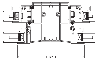
4300 SINGLE HUNG INTERMEDIATE JAMB HORIZONTAL CROSS SECTION
