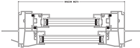
4300 SINGLE HUNG WITH J-CHANNEL HORIZONTAL CROSS SECTION
